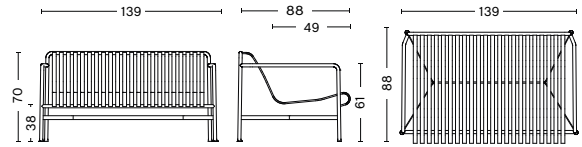
PALISSADE LOUNGE SOFA WIDTH 139 CM DEPTH 88 CM HEIGHT 70 CM SEAT HEIGHT 38 CM SEAT DEPTH 49 CM
